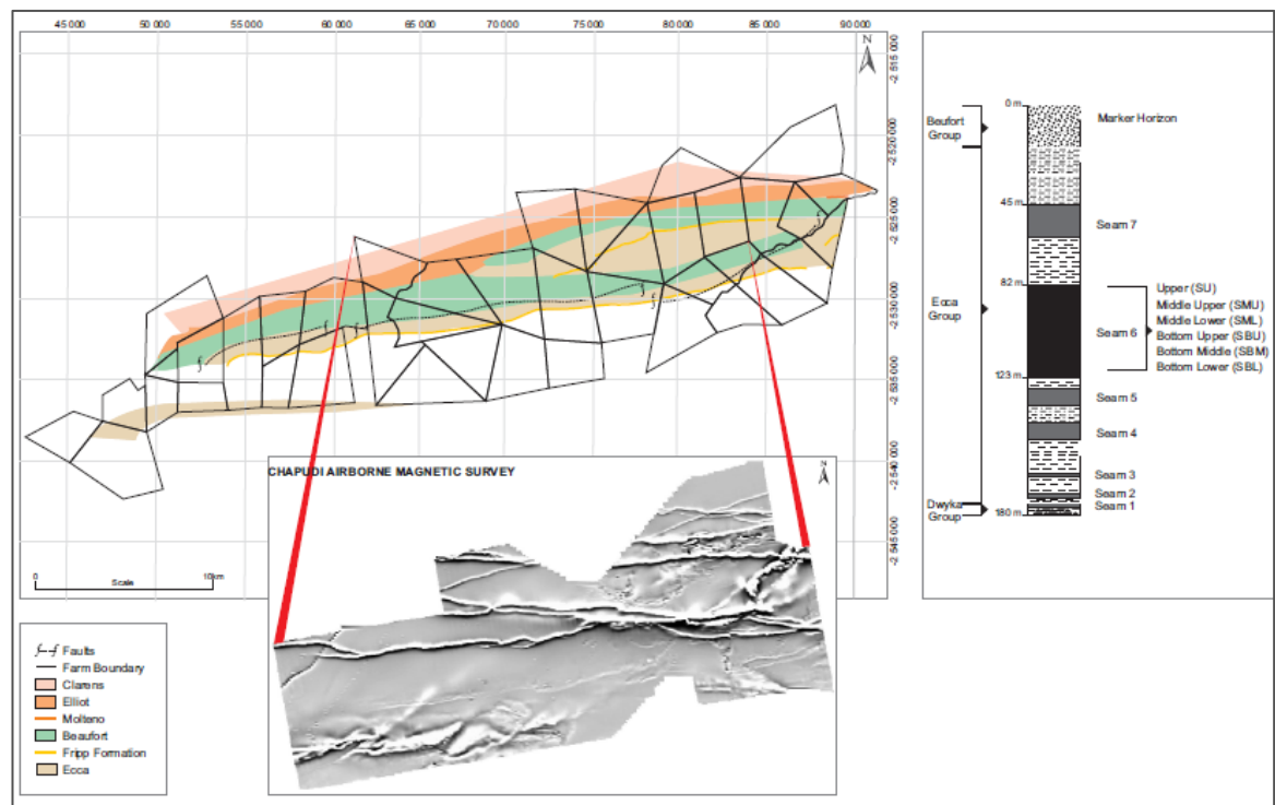
Figure 6.13: Chapudi Section – surface geology and typical stratigraphy
